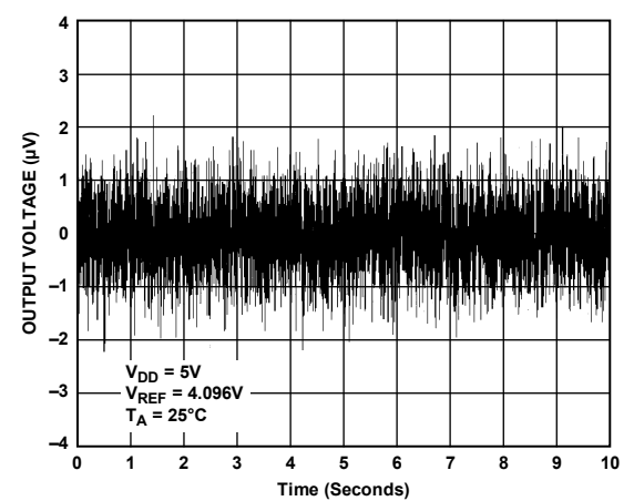
Figure 33. 1/f Noise
