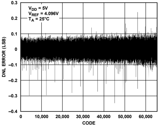
Figure 5. DNL Error vs. Code
