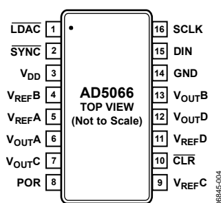
Figure 3. Pin Configuration
