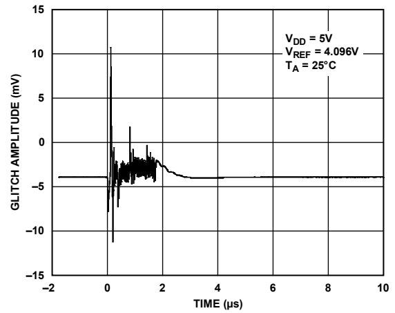
Figure 31. Digital Crosstalk
