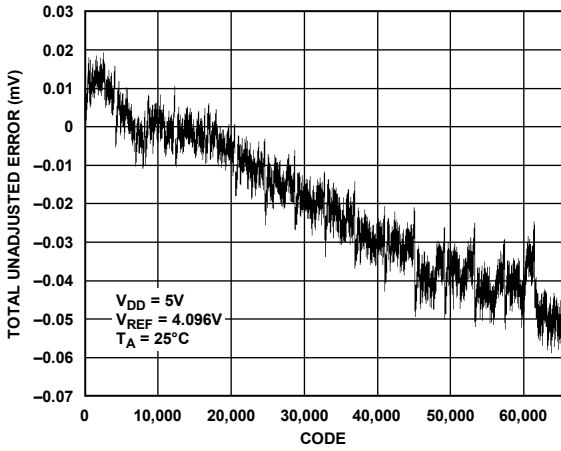
Figure 6. Total Unadjusted Error vs. Code
