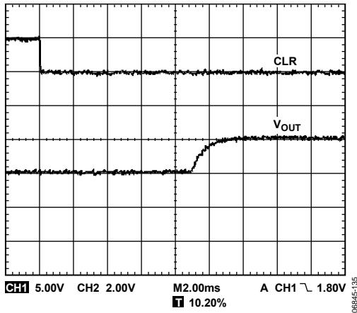
Figure 35. Hardware \overline{CLR}
