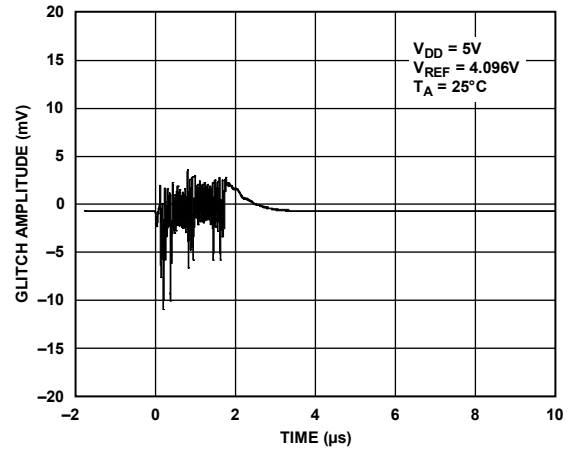
Figure 32. DAC-to-DAC Crosstalk
