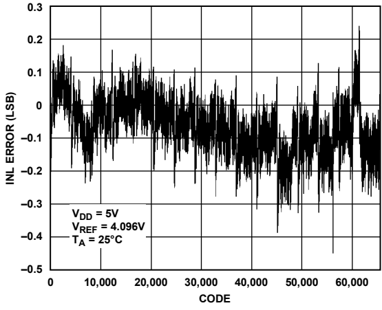
Figure 4. INL Error vs. Code
